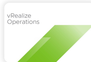
vRealize Operations
