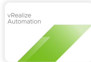
vRealize Automation
